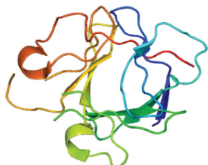
3D rendering of the structure of Keratinocyte Growth Factor.
